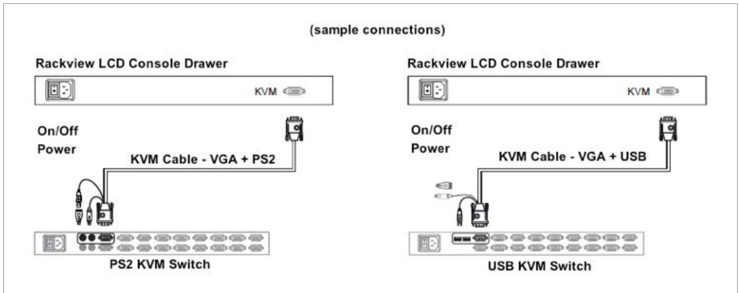
Figure 5. RackView cable connectivity
