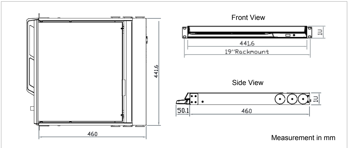
Figure 9. RackView chassis dimensions
