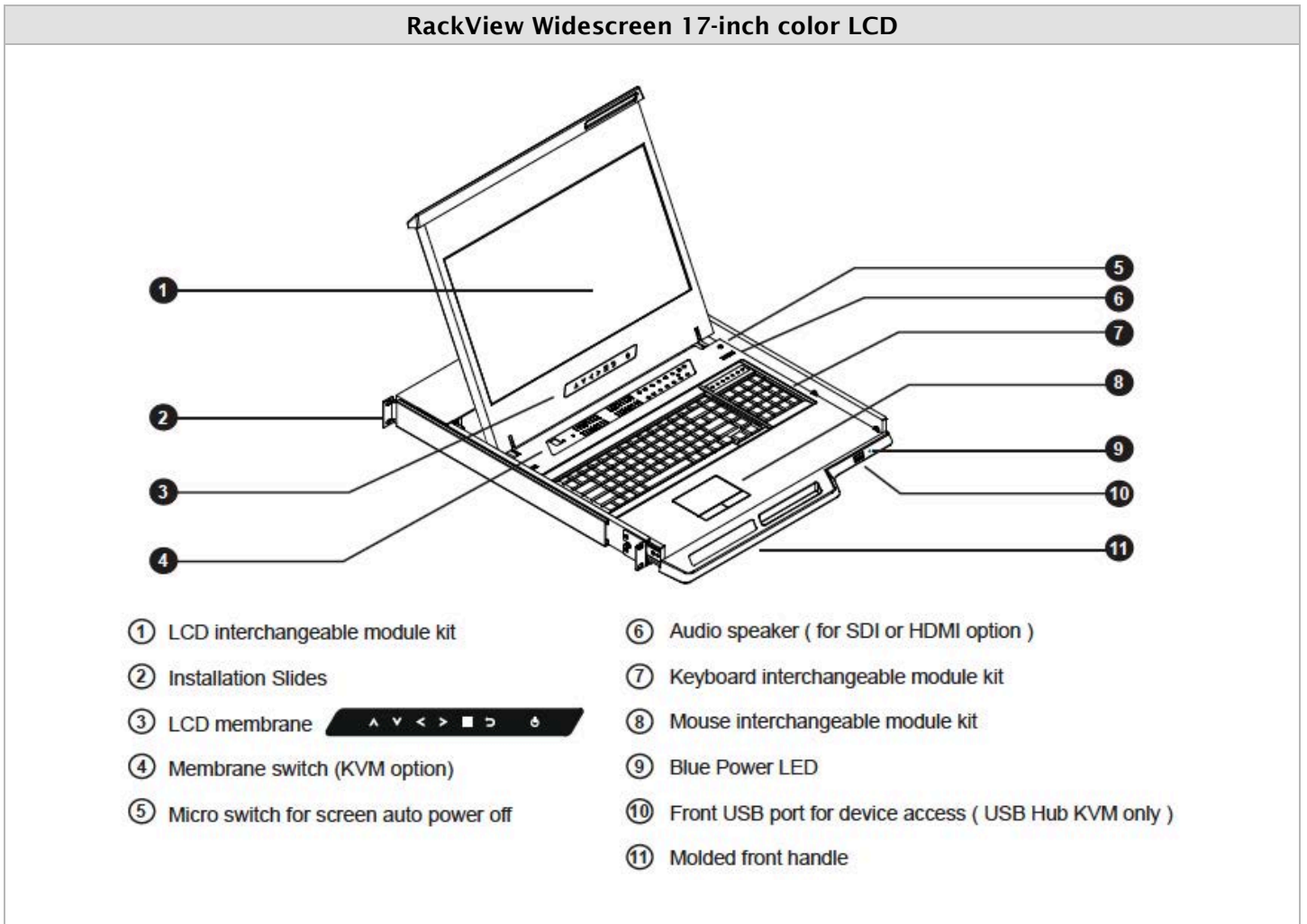
Figure 1. RackView product layout - key features
